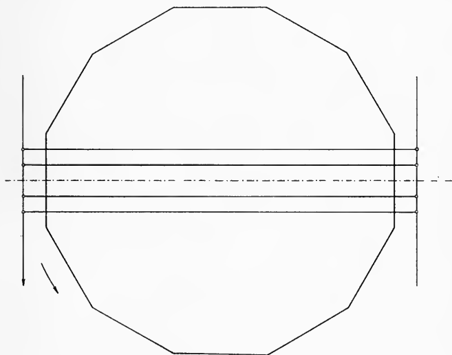
FIG. 3. Position of the rotating prism, two faces vertical to the optical axis.
